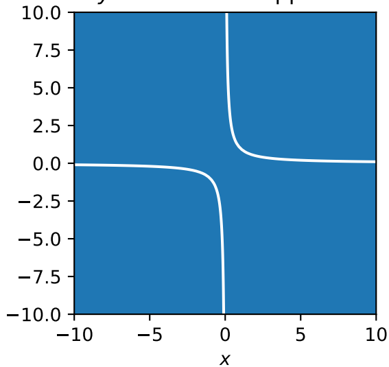
xy \neq 1 : Second approach
