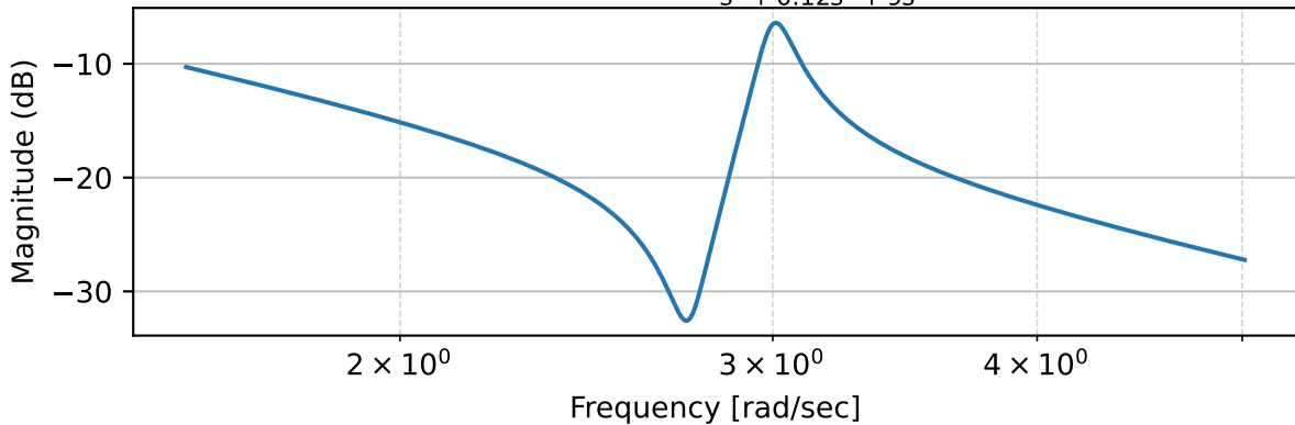
Bode Plot of \frac{s^2 + 0.1s + 7.5}{s^4 + 0.12s^3 + 9s^2}
